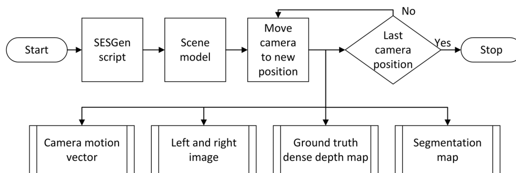
Fig. 5 Block diagram illustrating generation of motion vectors, images, depth, and segmentation maps in the stereovision egomotion sequence generator (SESGen) software tool.
