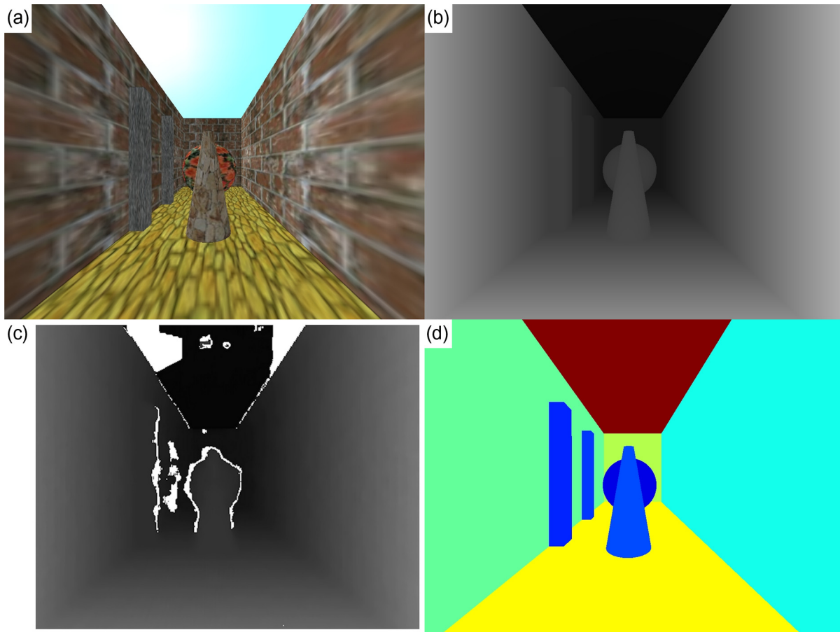
Fig. 6 A 3-D test scene defined by the script listed in Fig. 5: (a) 3-D test scene, (b) ground-truth disparity map computed with subpixel accuracy, (c) disparity map obtained using sum of absolute difference (SAD) (block matching) criterion, (d) scene segmented into 3-D objects and flat quadrangles positioned in 3-D space.
