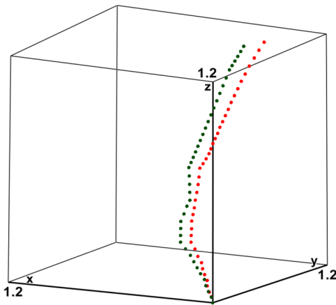
Fig. 8 Visualization of 3-D egomotion paths of the stereovision system: green dots (on the left) indicate a sequence of camera positions defined from the SESGen tool and the red dots (on the right) denote a sequence of camera positions computed from the tested visual odometry (VO) algorithm.
