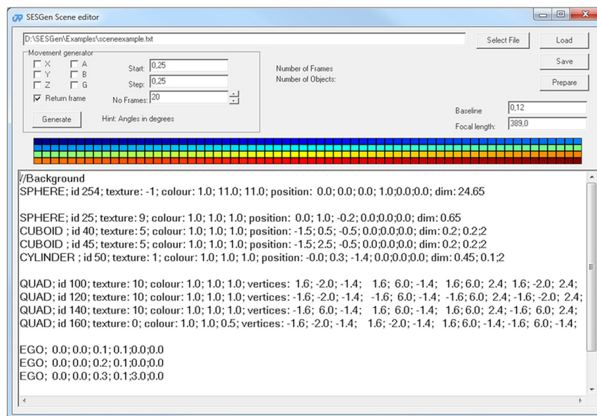
Fig. 7 View of the program window for defining and editing three-dimensional (3-D) scenes and ego-motion paths (see the SESGen User Guide 26 for a complete explanation of the script keywords and parameters).
