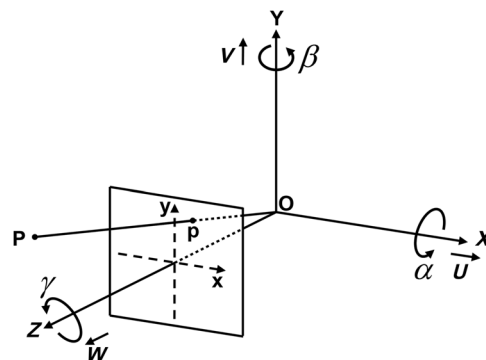
Fig. 1 The OXYZ frame of reference and the image coordinate system oxy with the indicated translation motion parameters ( U, V, W ) and rotation motion parameters ( \alpha, \beta, \gamma ).
