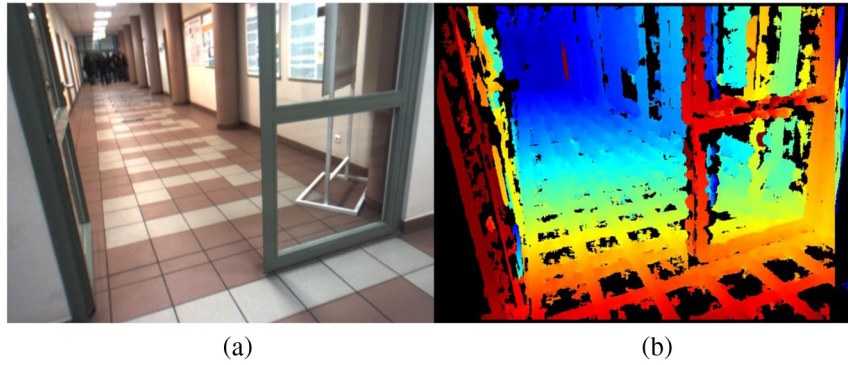
Fig. 2 (a) Image taken by the right camera of a stereovision system after compensation of geometric distortions and (b) the corresponding disparity map displayed in pseudocolors. Black regions denote areas of the map for which disparity could not be calculated with sufficient confidence.
