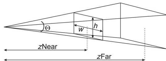
Fig. 4 A viewing frustum defining the field and depth of view for a perspective camera model.
